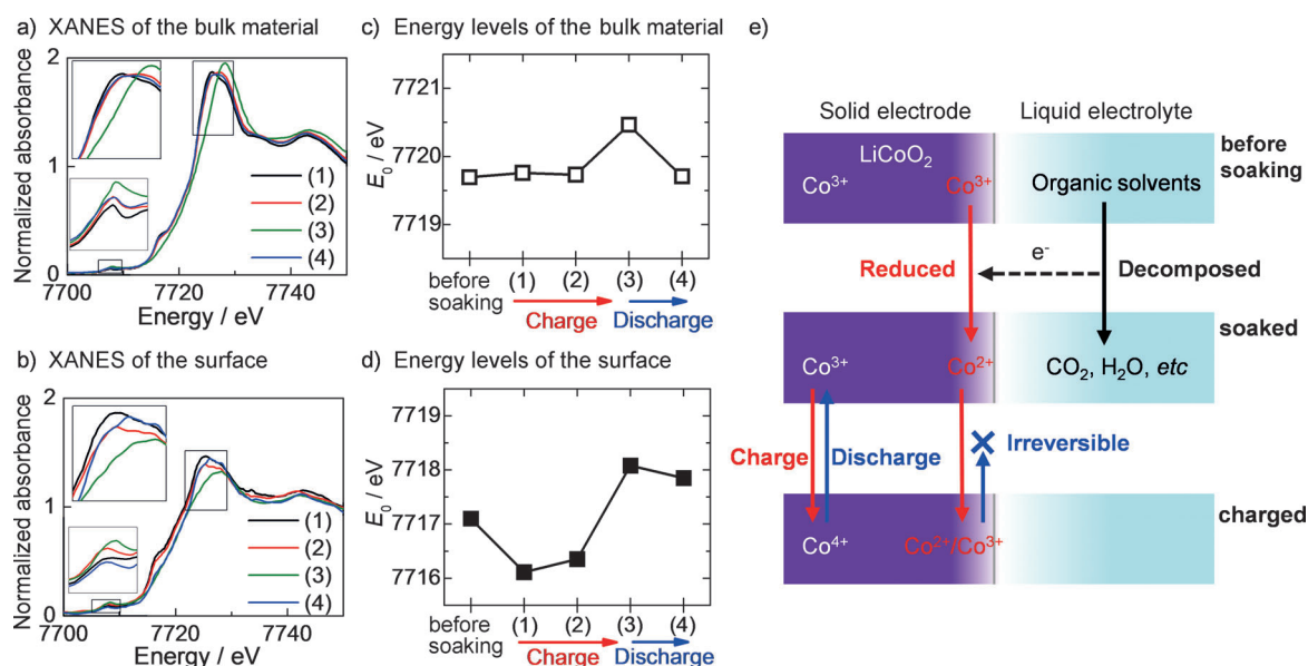
Figure 4. a)–d) Co K-edge XANES spectra of the LiCoO 2 film measured at points (1)–(4) in Figure 1 by applying a voltage and measuring the corresponding absorption energy levels of the bulk material (a, c) and the surface (b, d), respectively. e) The proposed reaction of the initial degradation that occurs at the electrode/electrolyte nano-interface.
